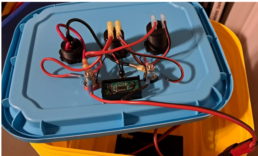
Wiring harness view of cat litter battery box.
